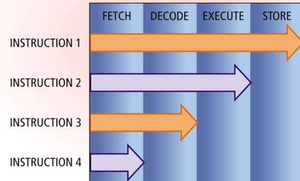
MACHINE CYCLE (with pipelining):
